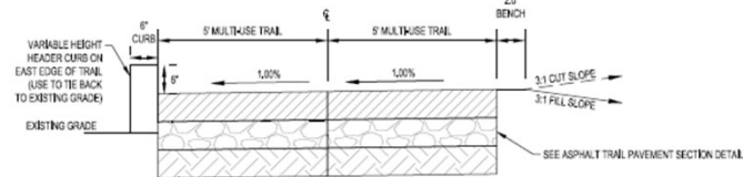
TRAIL TYPICAL SECTION LEFT SLOPING - 10' TRAIL (1%) WITH BENCH & 3:1 TIE NOT TO SCALE
