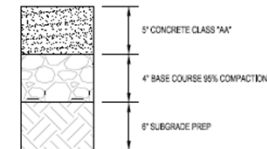
CONCRETE PAVEMENT TRAIL SECTION DETAIL NOT TO SCALE
