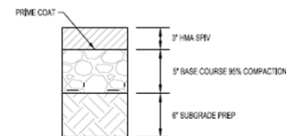
ASPHALT TRAIL PAVEMENT SECTION DETAIL NOT TO SCALE
